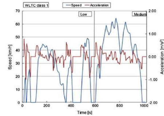
Figure 2. WLTC Class 1 v3.2 Speed and acceleration profiles.
