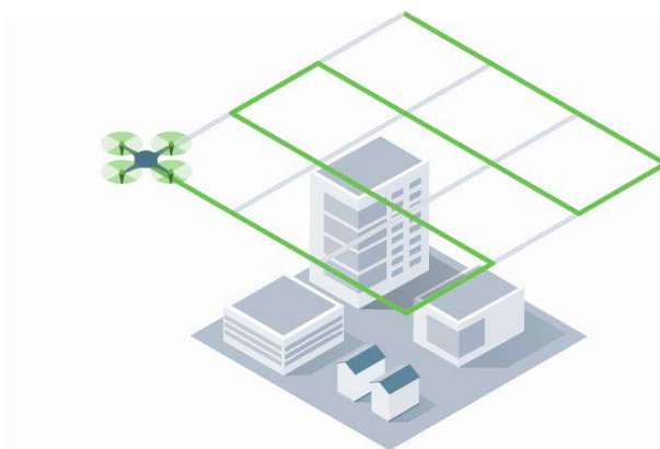
Figure 10. Double grid flight plan
