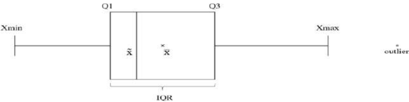
Figure 1. Box Plot
