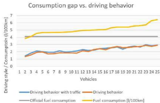
Figure 5. Relation between driving behavior w/o traffic and consumption gap.
