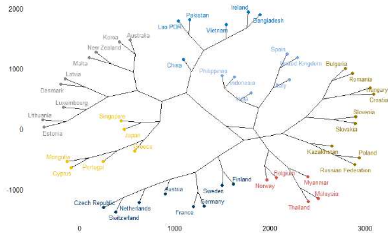
Figure 3. Phylogenetic Tree.
